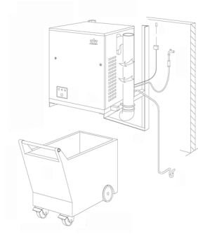
Ice production into an ice trolley
